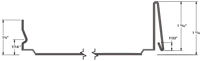
1.5" Snap Lock Panel SS450SL
