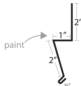
Counter Flashing
