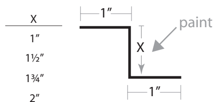
Z-Closure
